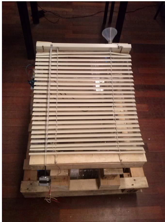
Figure 30. Stepper motor location
