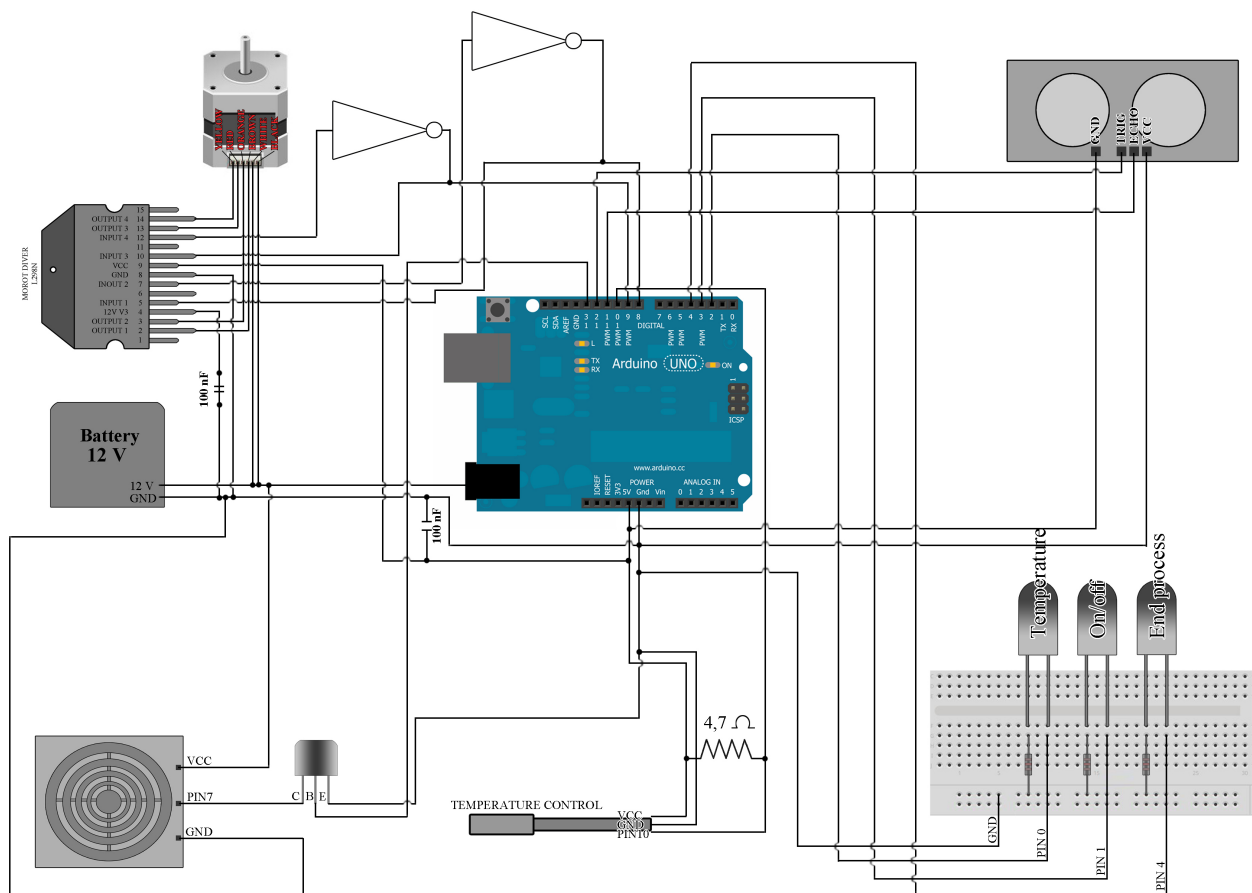
Figure 12. Electrical chart
