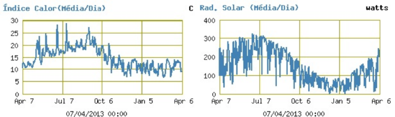
Figure 22. Solar radiation and Heat index diagrams [46].
