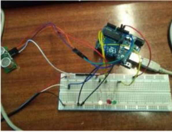
Figure 29. Connected electrical circuit
