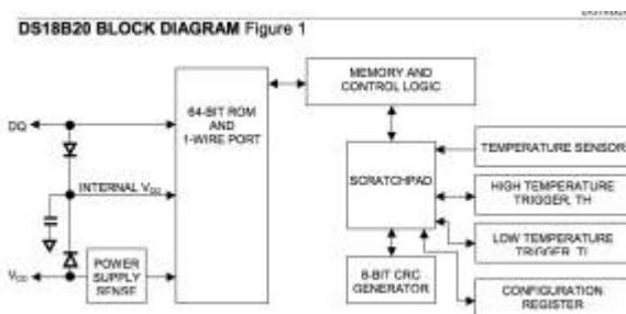
Figure 6. Block diagram for temperature sensor [7]
