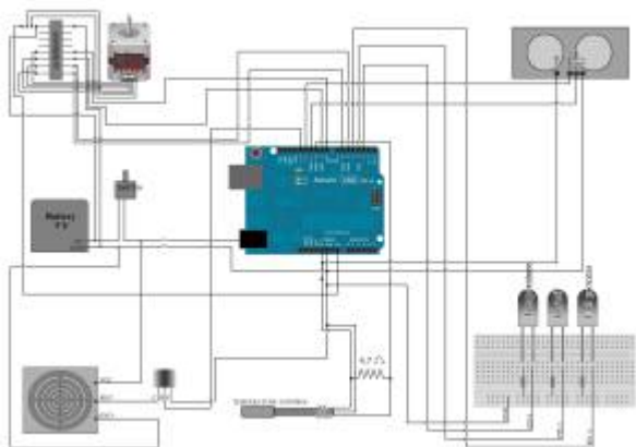
Figure 28. Electrical chart
