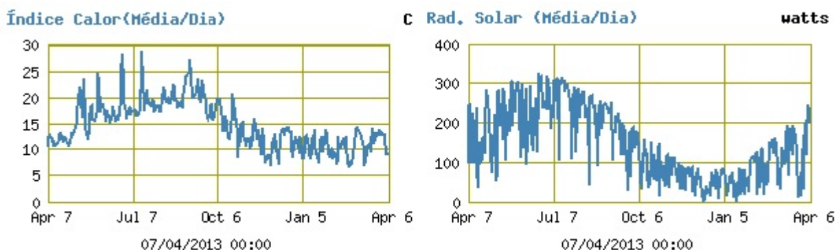
Figure 45. Solar radiation and Heat index diagrams [46]
