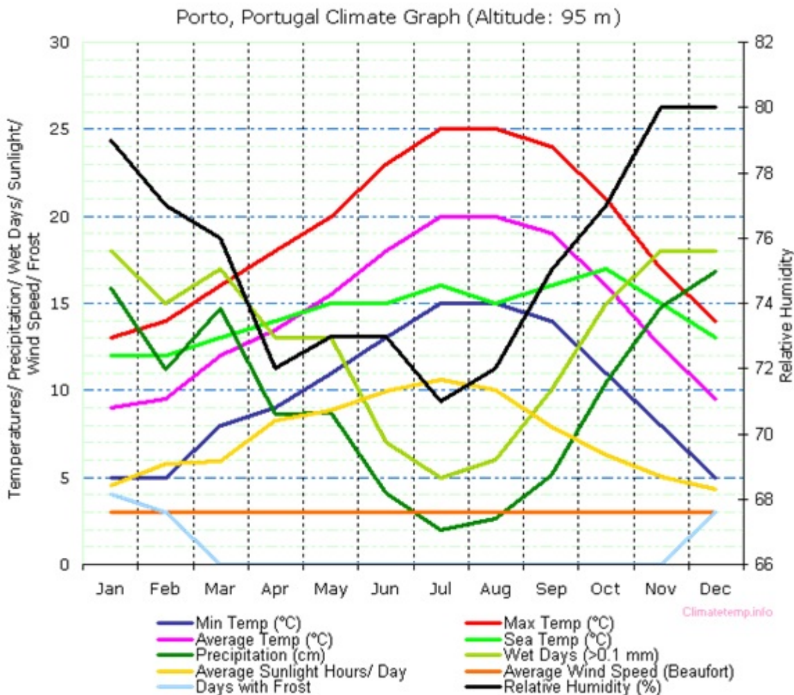
Figure 46. Climate graph for Porto [47]
