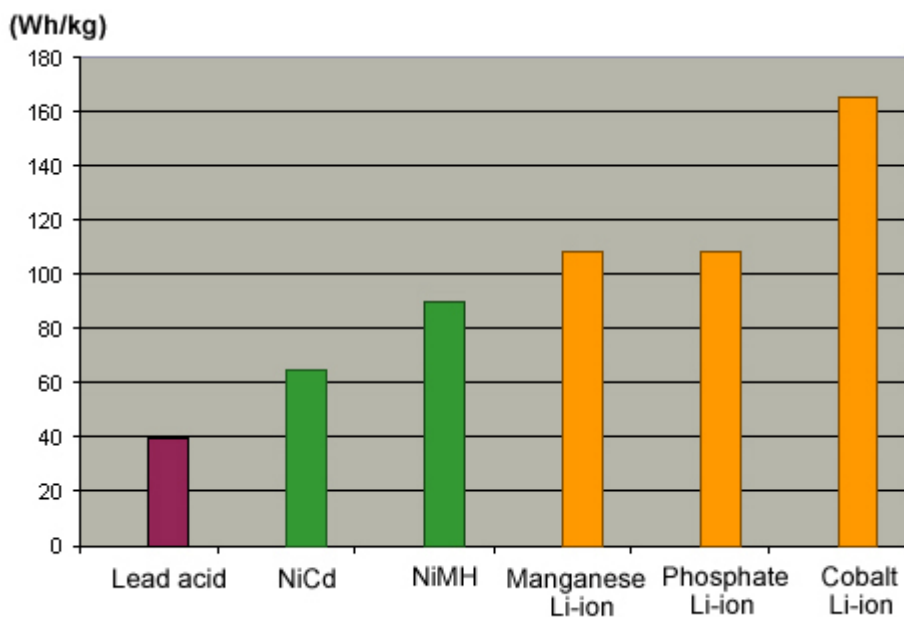
Figure 17. Energy density performance of batteries [13]
